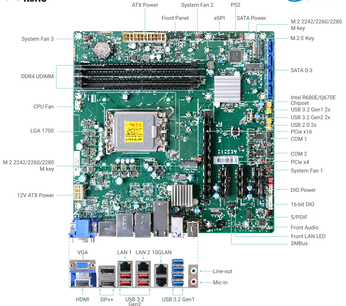
Top View
